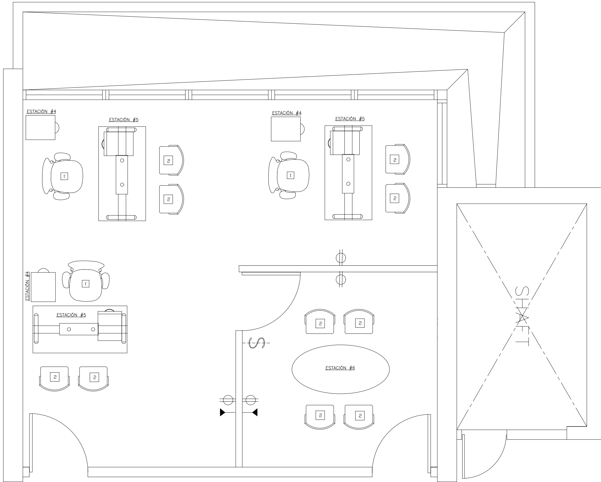
MOBILIARIO ESCALA: 3/4" = 1'-0"
