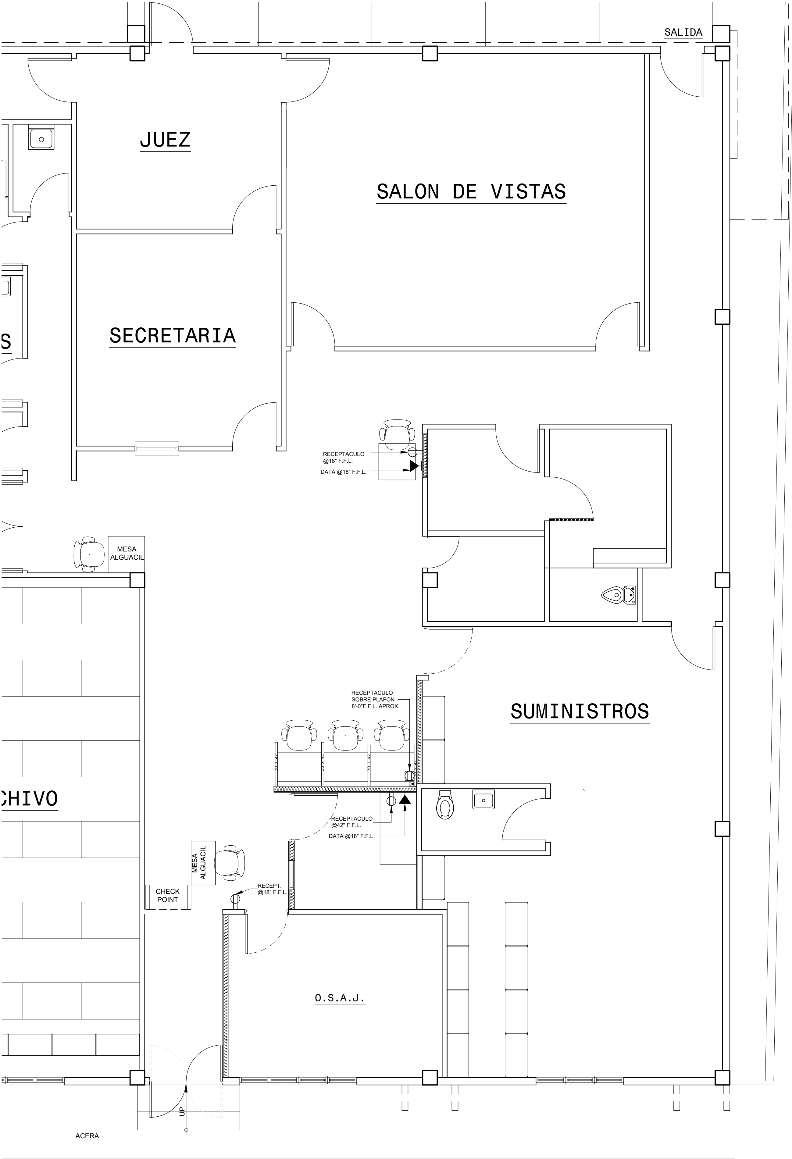
PLANTA ELECTRICA SUMAC MUNICIPAL C/AIBONITO SCALE: 1/4"=1'-0"
