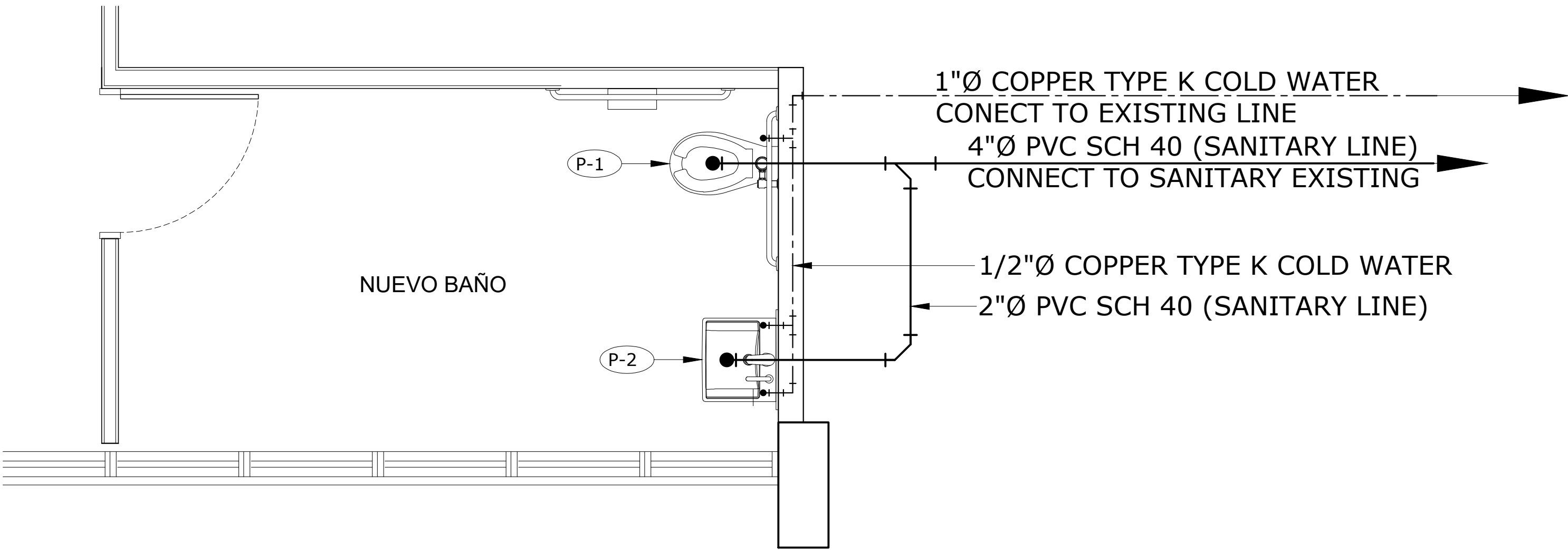
PLUMBING FLOOR PLAN (new bath) SECOND FLOOR PLAN (edificio principal) SCALE: 1/2"=1'-0"
