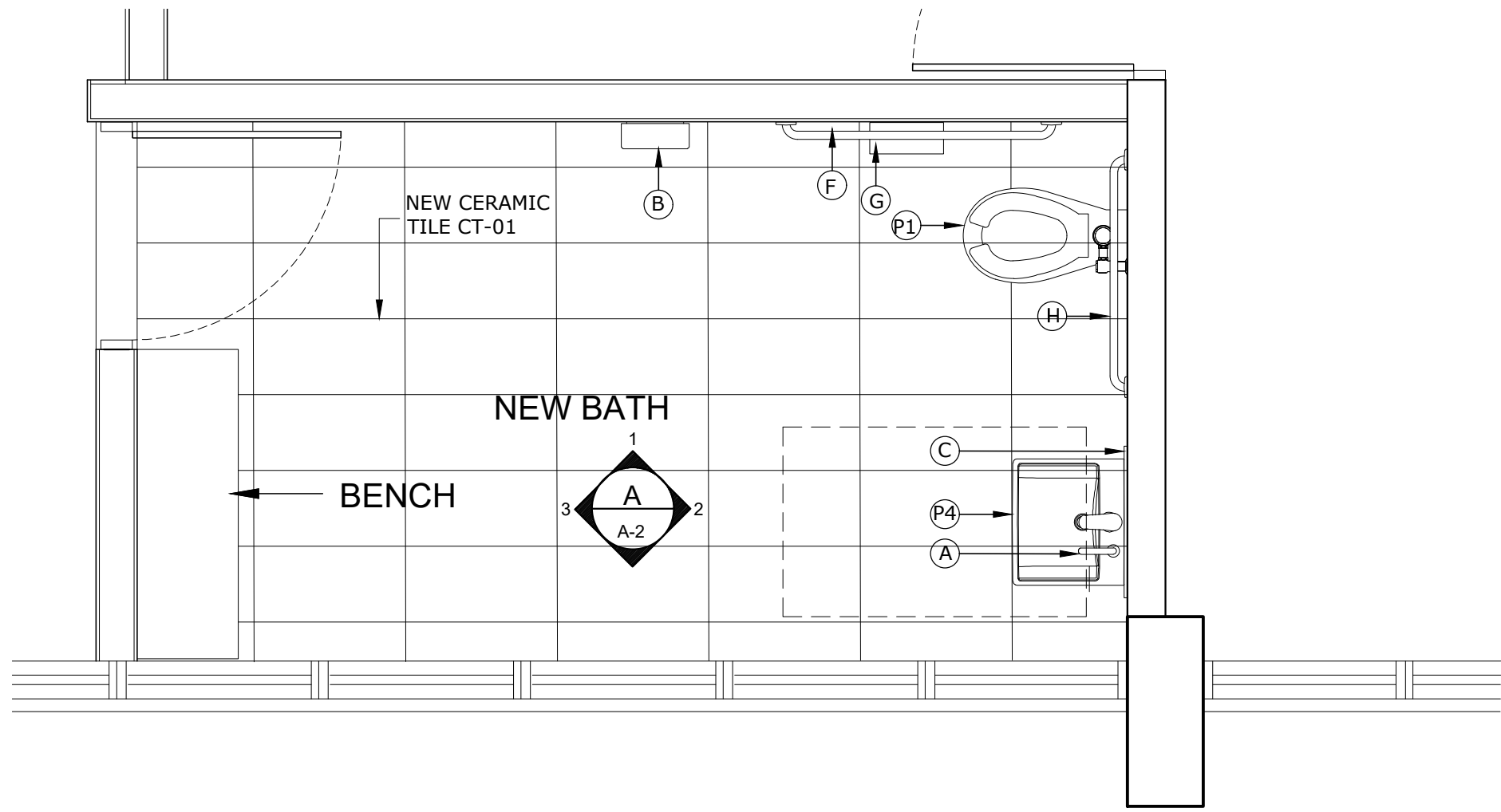
NEW BATH OFFICE SR. JUEZ COLON SECOND FLOOR PLAN (edificio principal) SCALE: 1/2"=1'-0"
