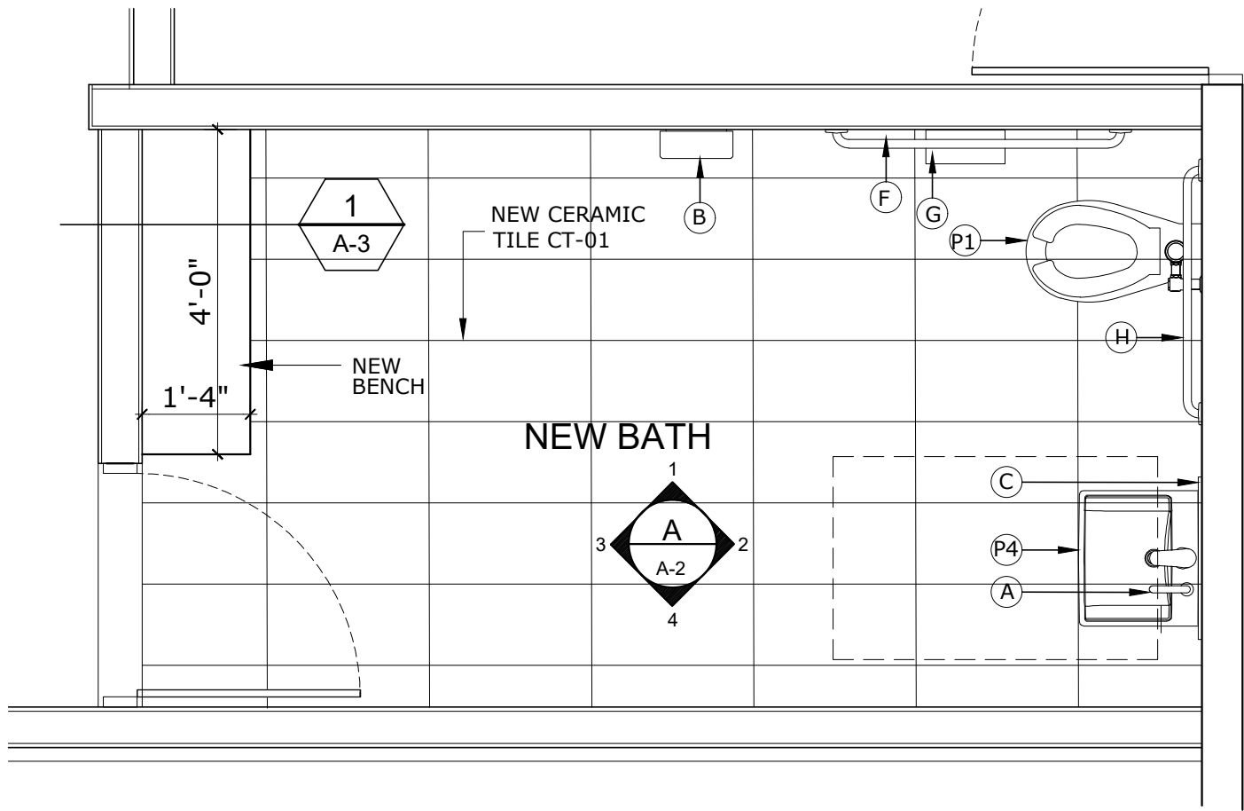
NEW BATH OFFICE SR. JUEZ COLON SECOND FLOOR PLAN (edificio principal) SCALE: 1/2"=1'-0"
