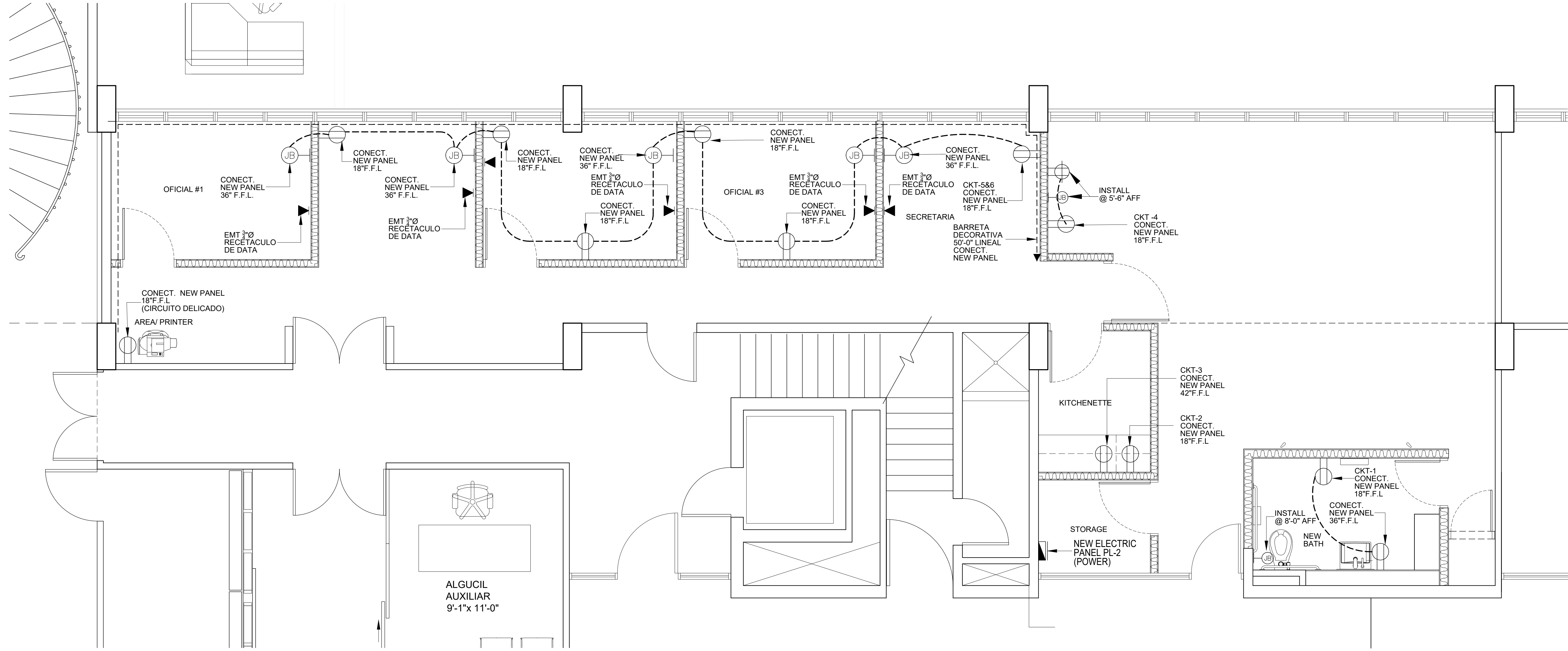
POWER FLOOR PLAN, NEW OFFICE SECOND FLOOR PLAN (edificio principal)
