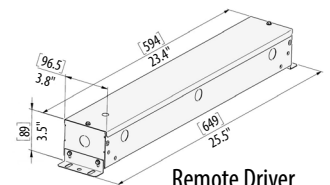
Remote Driver Box/Emergency Battery Box
