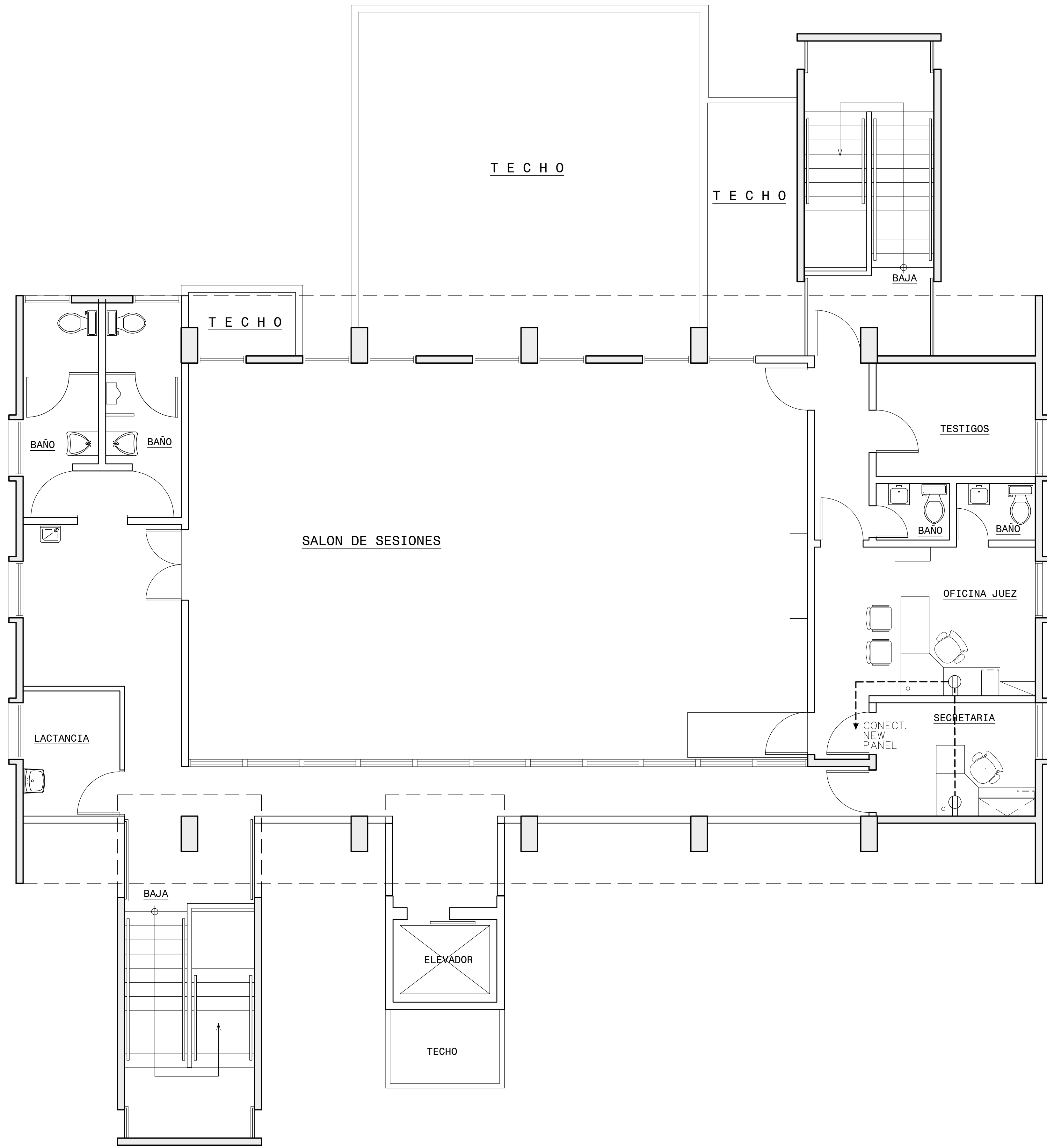
PLANO MODULACION FIRST FLOOR LEVEL SCALE: 1/4"=1'-0"
