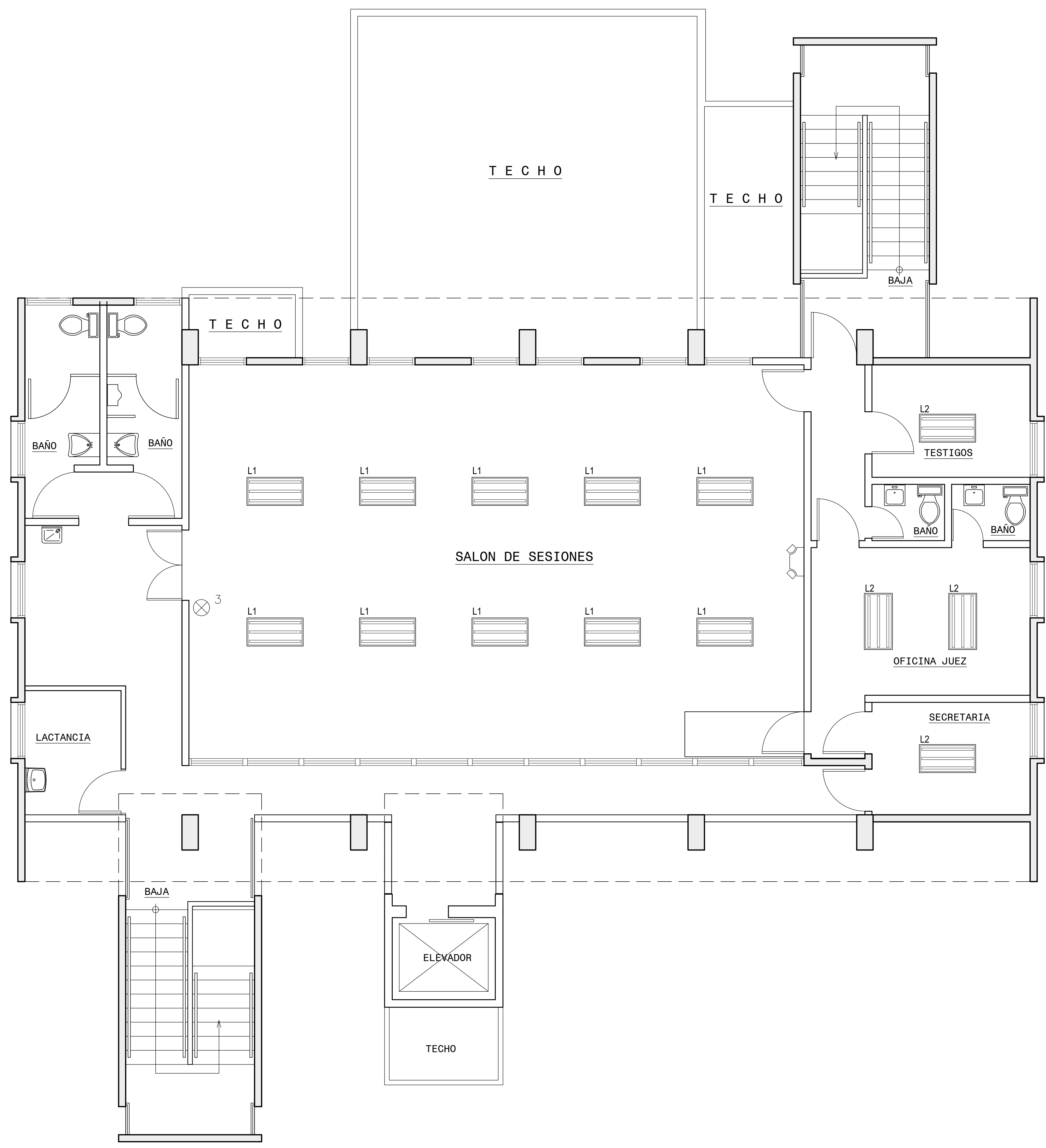
EXISTING LIGHTING 2ND FLOOR SCALE: 1/4"=1'-0"
